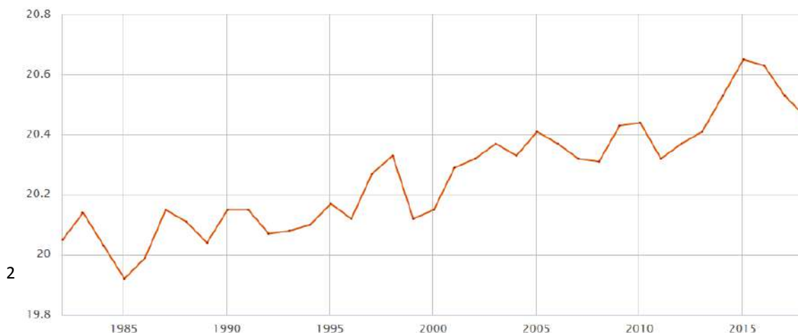
World (60°S–60°N) Annual Sea Surface Temperature (°C)
